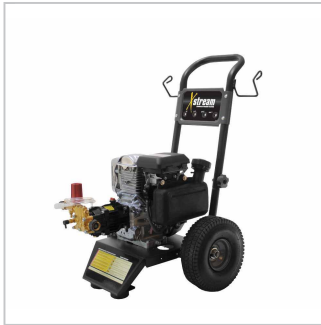
WASHER, GAS 5HP 2500PSI, 2.4GPM, HONDA, Code : BPS / 856 / X2005HWX
